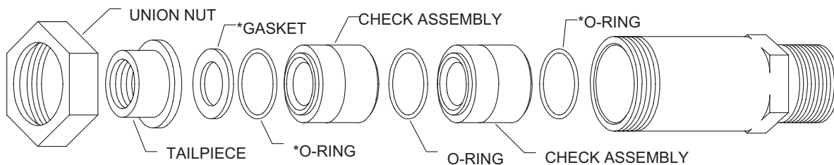
METER SETTER INSTALLATION
