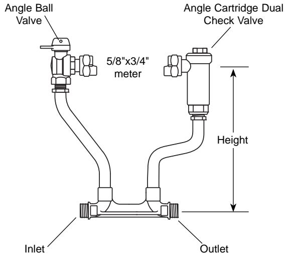
Male Threads for Pack Joint Assemblies (PJAx-1x-NL)
