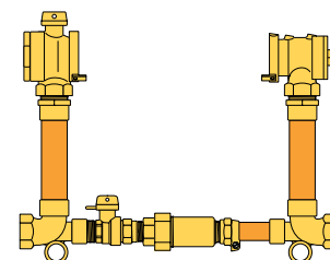
Shown with cartridge dual check valve in by-pass. See information below to order this feature.
