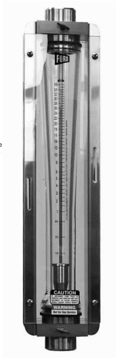
The Testerate Indicator has a length of 17-5/8". Both ends are tapped 1" I.P. thread.
