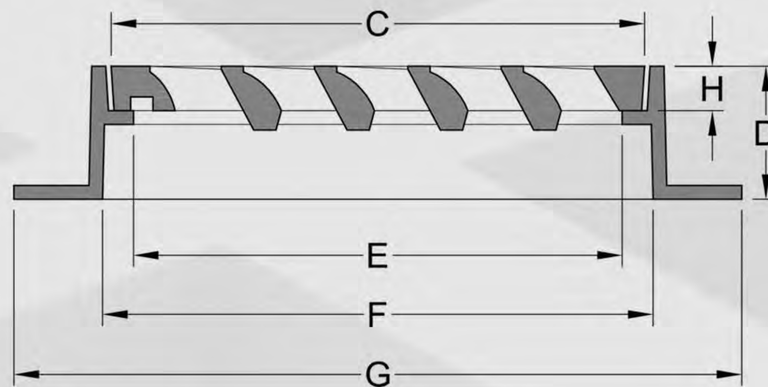
4 FLANGE FRAME WITH CASCADE GRATE
