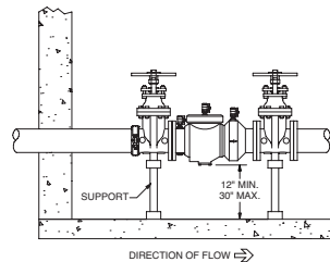
INDOOR INSTALLATION (350GF)
